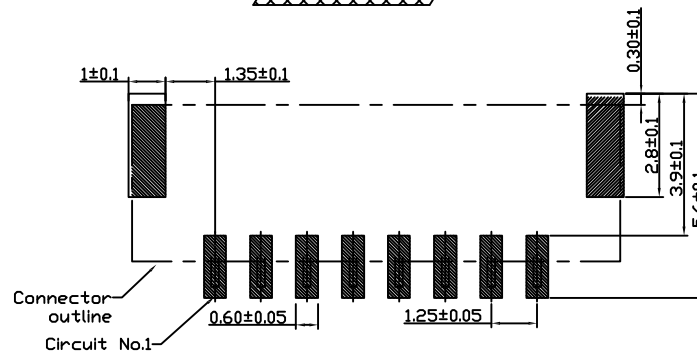
PCB LAYOUT
